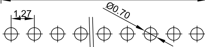
PCB LAYOUT
